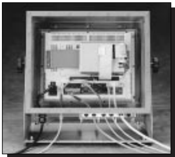
Unique cable entry design allows for easy cable installation. (No need to cut off connectors and then re-splice.)
