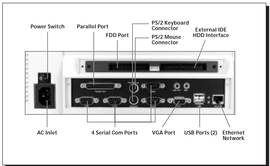
A standard PS/2 style keyboard can be quickly attached via an external keyboard port.
